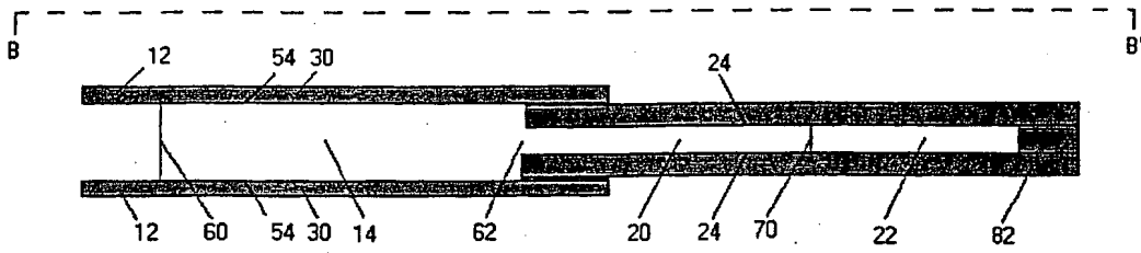
Cross Section Along Line B-B' of FIG. 4
